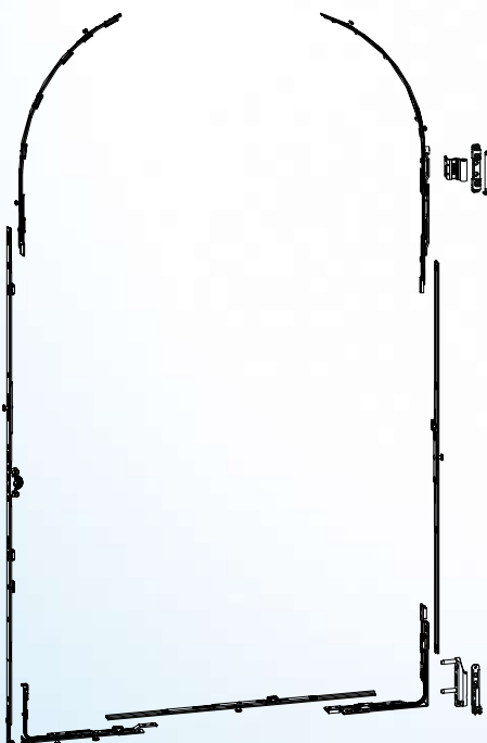
Round arch head window
